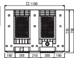
< "L" TYPE BLOCK부착시 >
